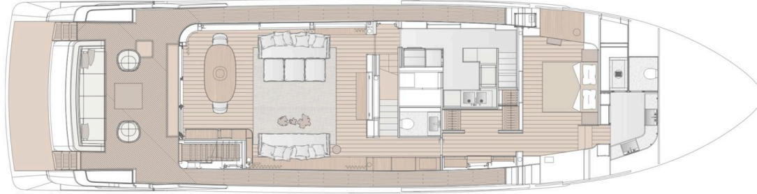
2.2.4.5.Lower Deck
