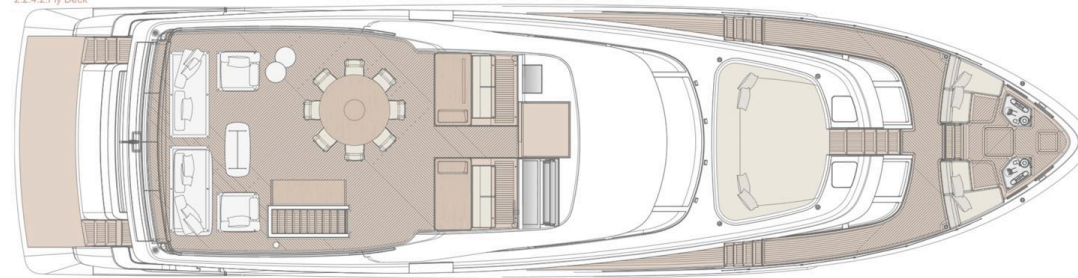
2.2.4.2.Fly Deck
