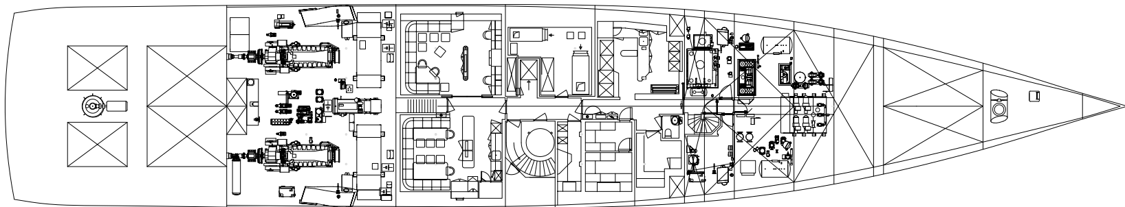
Tank Deck
