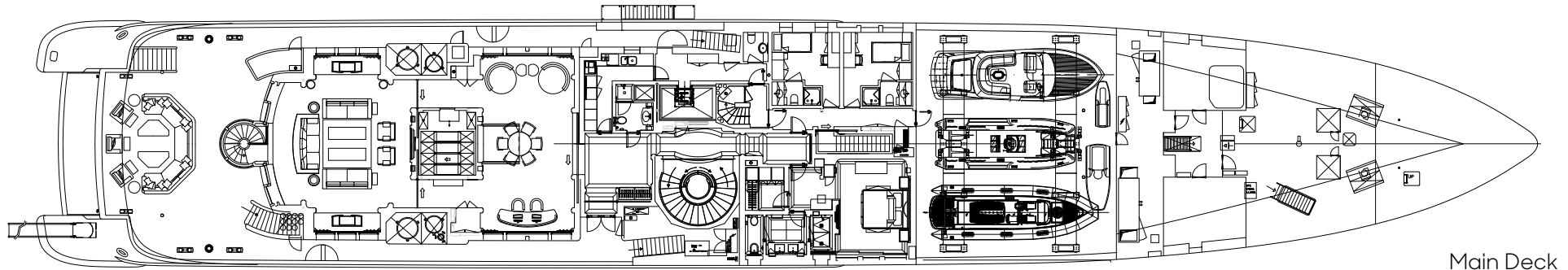
Main Deck
